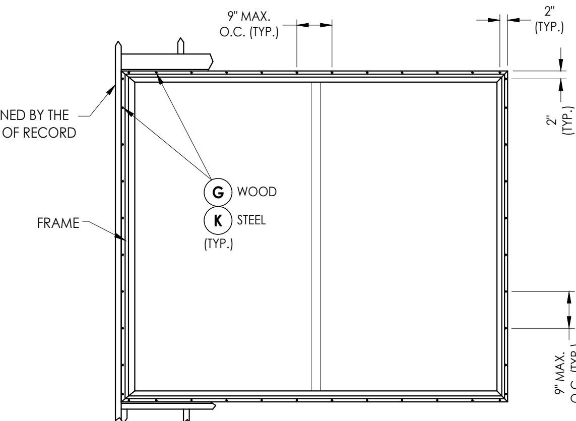
FRAME ANCHORING (2X Stud, Steel Stud)
